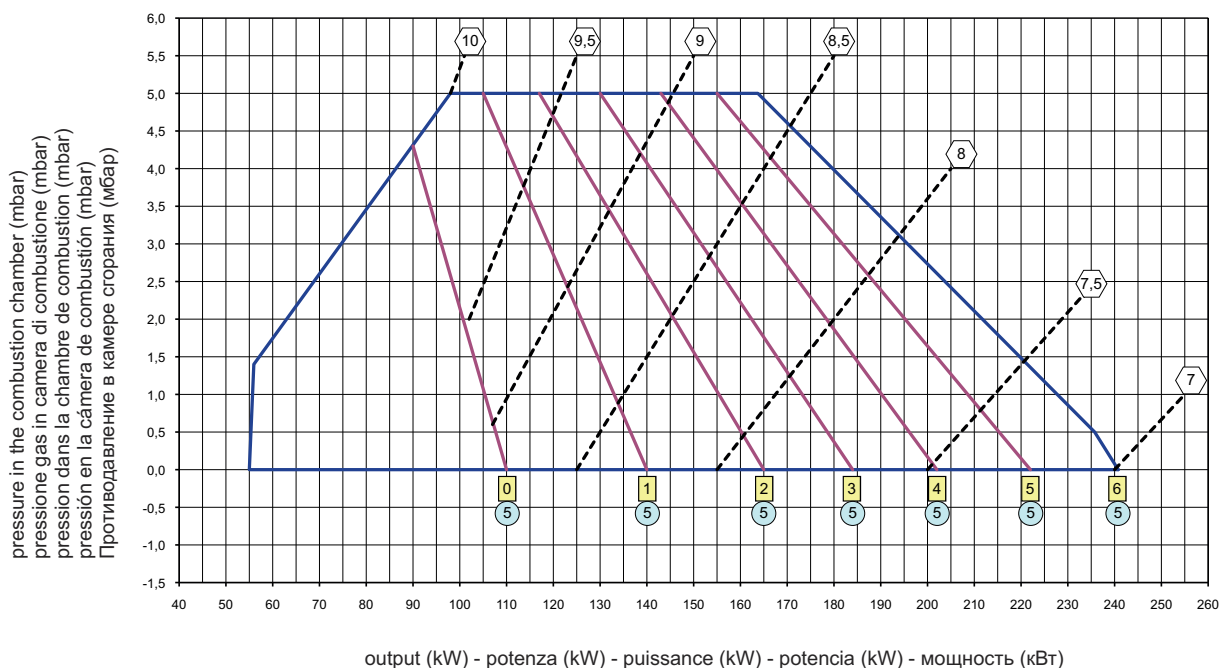
MAX GAS 250 P LPG
