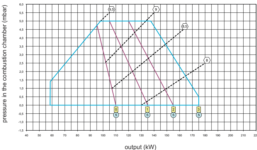
MAX GAS 170 P NATURAL GAS
