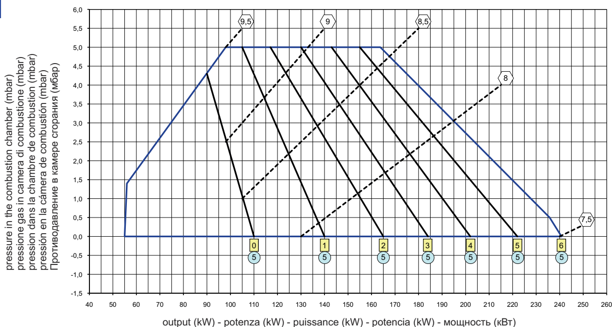
MAX GAS 250 P NATURAL GAS
